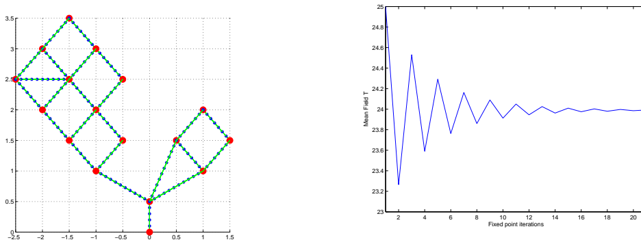
Figure 3: Left: Graph configuration. Right: approximated mean field time T_2 vs. fixed point iterations, computed by Algorithm 1
