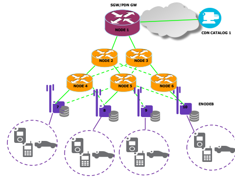
Figure 1: Down-scaled backhaul model topology used in the demonstration.
