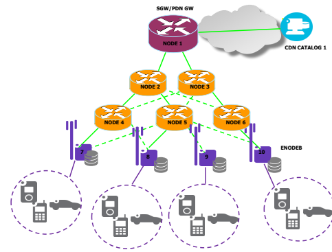
Figure 1: Down-scaled backhaul model topology used in the demonstration.
