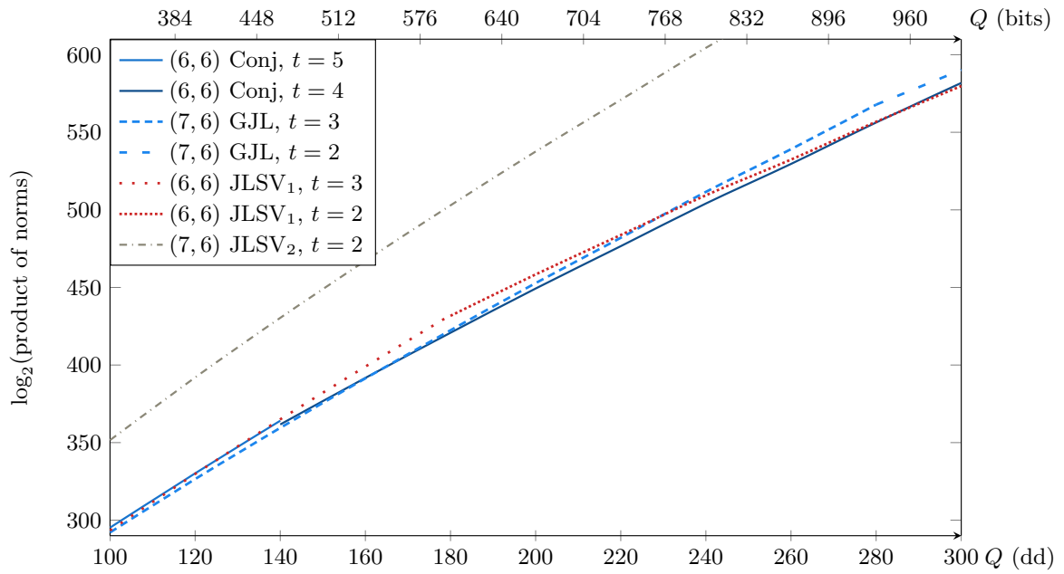
Fig. 6. Polynomials for \mathbb{F}_{p^6} .
