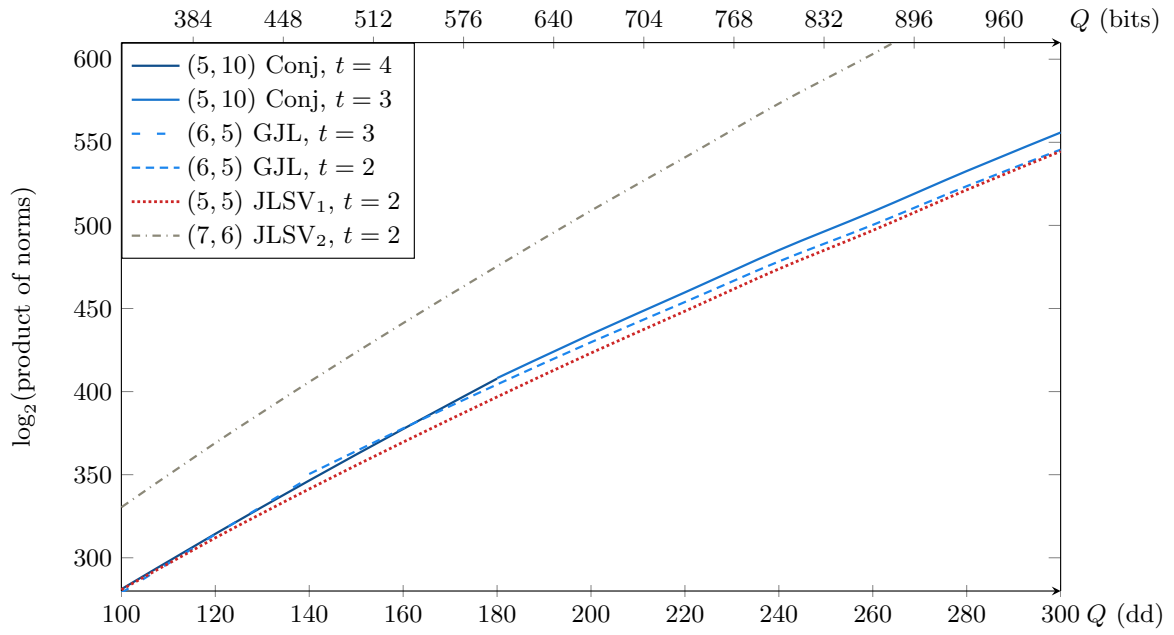
Fig. 5. Polynomials for \mathbb{F}_{p^5} .
