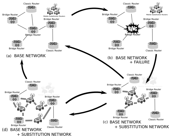
Fig. 1. Typical use case for a base network and a substitution network.
