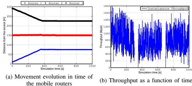
Fig. 5. One source, one destination, and three mobile routers.
