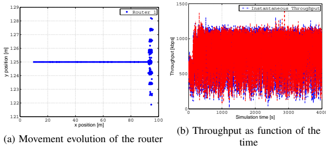
Fig. 8. Scenario two sources and one destination. Movement of the mobile router through the time and the corresponding throughput.
