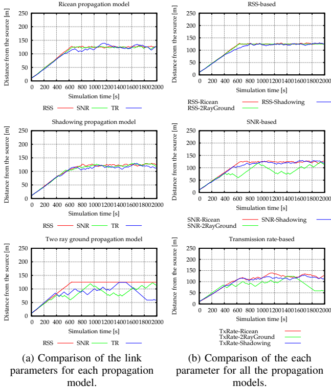
Fig. 10. Evaluation of APOLO under different propagation models. The movement of the mobile router as function of time.
