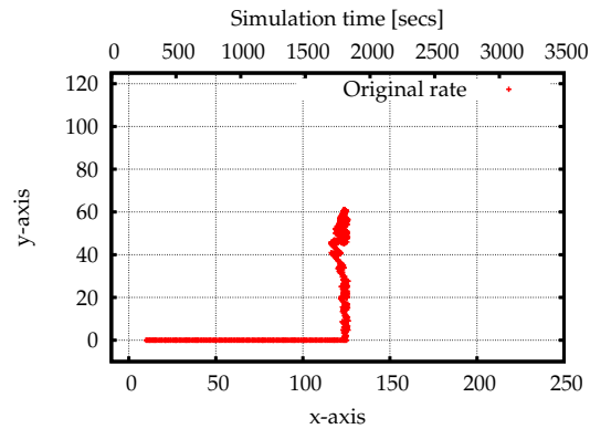
Fig. 9. Redeployment of a mobile router.
