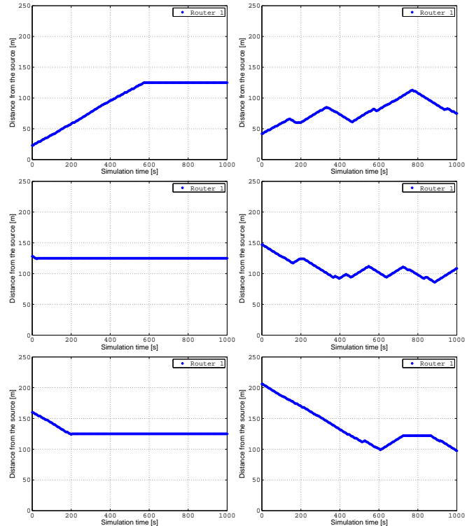
(a) Results by using the RSS as link metric (b) Results by using the SNR as link metric
