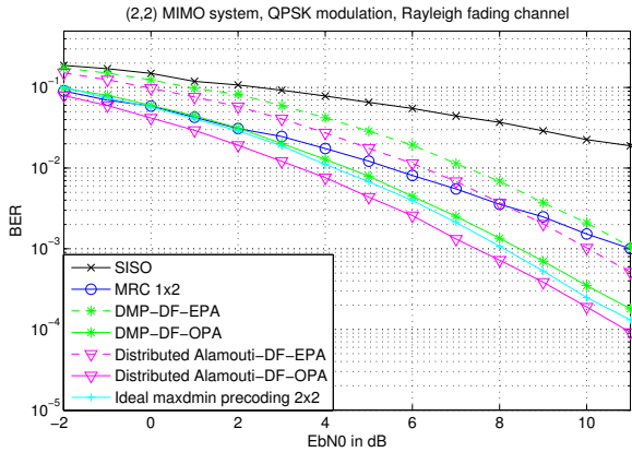
Fig. 2. BER performance comparison: DMP vs. traditional schemes
