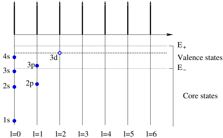
Figure 1: Sketch of the spectra of the operators H_z^{AA}|_{\mathcal{H}_l} and admissible energy window \Delta E = (E_-, E_+) for the copper atom ( z = 29 ). The energy scale is arbitrary. The actual values of the energy levels are the following: \epsilon_{z,1,0} \simeq -312.78 Ha (1s), \epsilon_{z,2,0} \simeq -36.42 Ha (2s), \epsilon_{z,1,1} \simeq -31.57 Ha (2p), \epsilon_{z,3,0} \simeq -3.716 Ha (3s), \epsilon_{z,2,1} \simeq -2.294 Ha (3p), \epsilon_{z,4,0} \simeq -5.540 \times 10^{-2} Ha (4s), \epsilon_{z,F}^0 = \epsilon_{z,1,2} \simeq -1.371 \times 10^{-2} Ha (3d). The self-consistent Hartree Hamiltonian H_z^{AA} seems to have no negative eigenvalue above the Fermi level \epsilon_{z,F}^0 .
