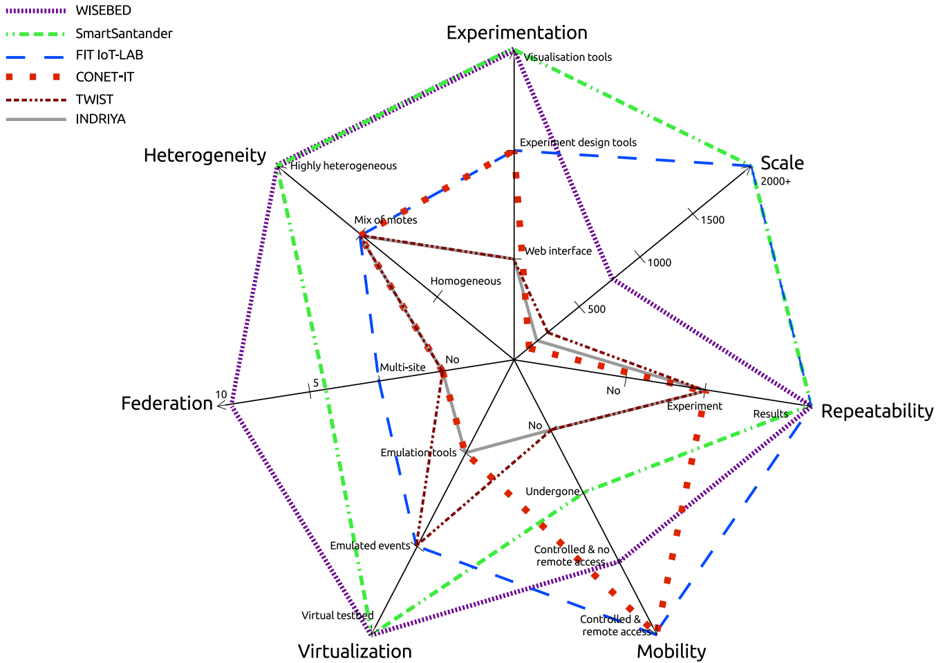
Fig. 3: Overview of the strengths and weaknesses of the main surveyed testbeds
