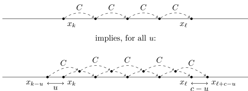
■ Figure 4 Illustration of the intuition for the construction of a behavior graph. Assume that the x_i 's form a path of length n from x_0 to x_n . If x_k and x_l are connected via a sequence of C 's, represented by the dashed edges, then for all u < c , there exists some intermediate nodes such that x_{k-u} and x_{l+c-u} are connected as shown in the picture.
