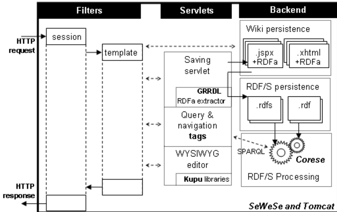
Fig 2. Architecture of SweetWiki in SeWeSe.
