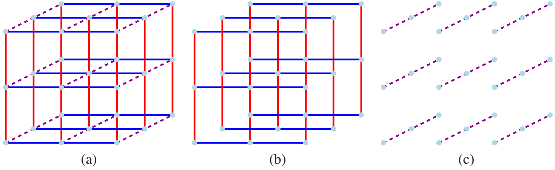
Figure 7: (a) Cut function F defined on a 3D-grid may be decomposed into: (b) F_1 represented by solid edges (red and blue) and (c) F_2 represented by dashed lines (magenta)
