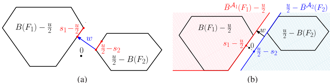
Figure 3: Closest point between two polytopes. (a) Output of Dykstra’s alternating projection algorithm for the TV problem, the pair (s_1, s_2) may not be unique while w = s_1 + s_2 - u is. (b) Dykstra’s alternating projection output for outer approximations.
