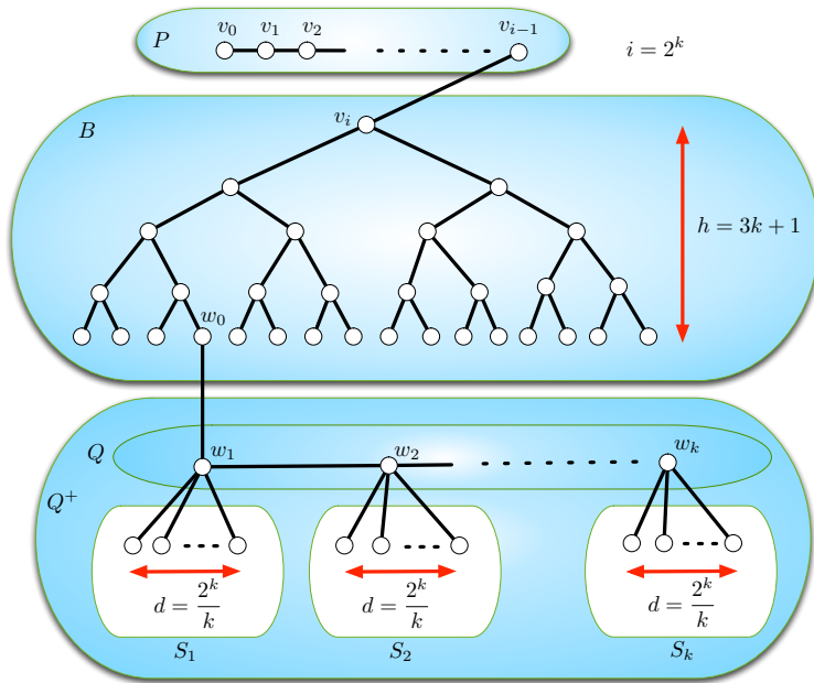
Figure 3: Tree T_k described in the proof of Theorem 10.
