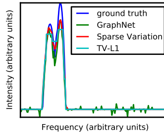
Fig. 1. Recovery for 1D spectroscopy. Note the blocky nature of the \text{TV-}\ell_1 solution, and the noise in the GraphNet estimation.
