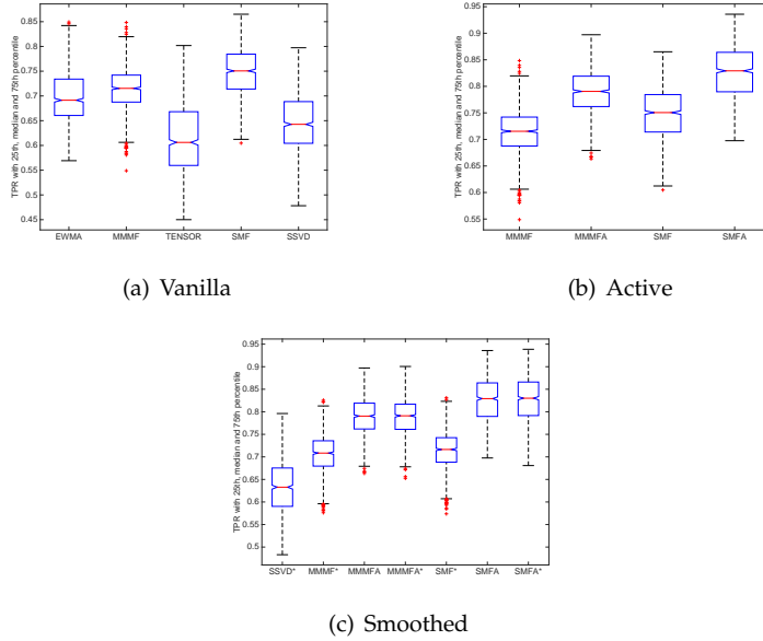
Figure 4: Descriptive statistics of methods on the non-curved dataset. Pairwise comparison shows significant difference at 95% confidence level, except for the impact of smoothing.
