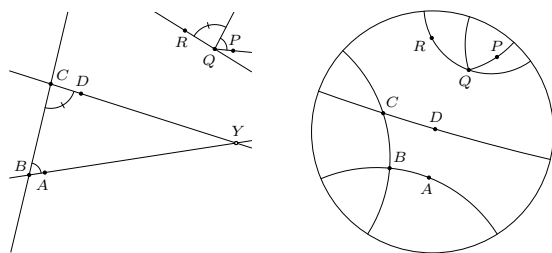
Fig. 38: Euclid’s parallel postulate (Postulate 20).
