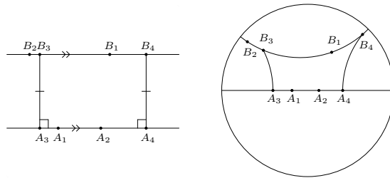
Fig. 26: Universal Posidonius' postulate (Postulate 11).
