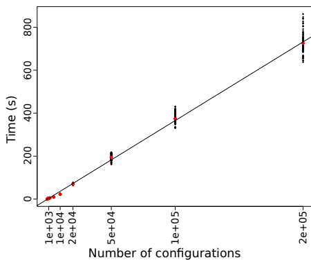
Figure 9: Scalability w.r.t the number of configurations
