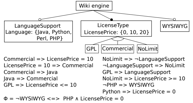
Figure 3: One possible attributed feature model for representing the configuration matrix in Figure 2
