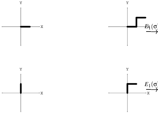
Fig. 6: The linear map associated with 1 \mapsto 121, 2 \mapsto 21
