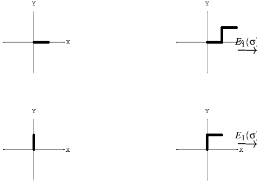
Fig. 6: The linear map associated with 1 \mapsto 121, 2 \mapsto 21
