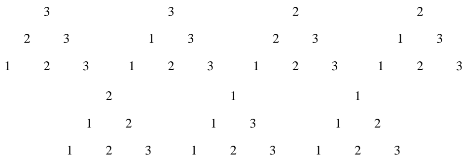
Figure 7: The seven monotone triangles of order 3.
