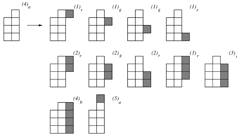
Fig. 5: The ECO operator for a polyomino in the class C_a .
