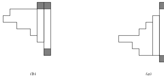
Fig. 2: Convex polyominoes in \mathcal{C}_b , (b), \mathcal{C}_a , (a).
