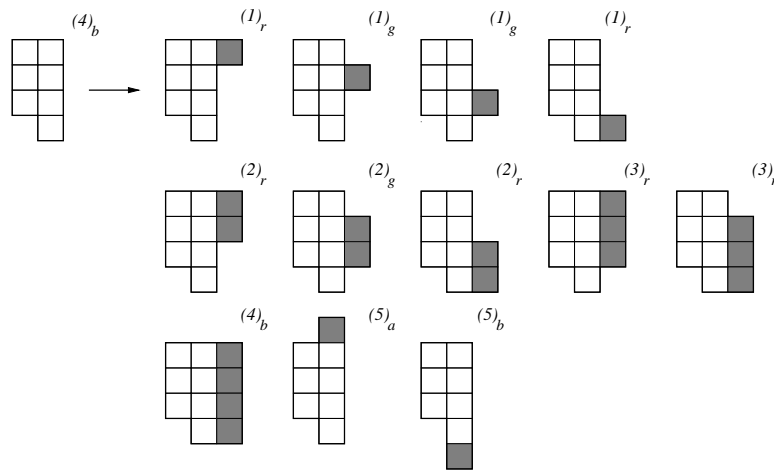
Fig. 4: The ECO operator for a polyomino in the class C_b .
