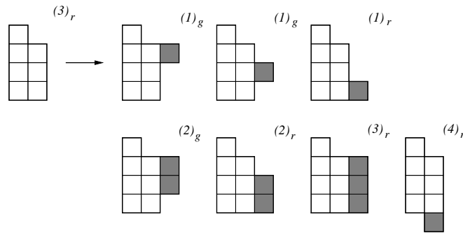
Fig. 6: The ECO operator for a polyomino in the class C_r .
