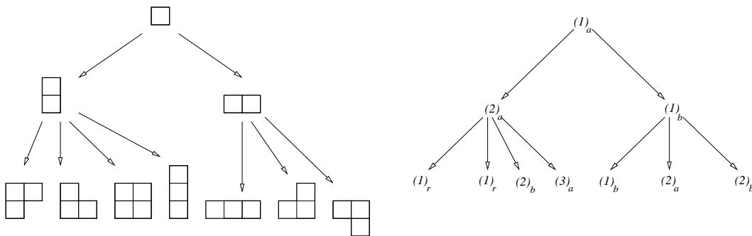
Fig. 8: (a) The first levels of the generating tree of the ECO operator \vartheta ; (b) the first levels of the generating tree of \Omega .
