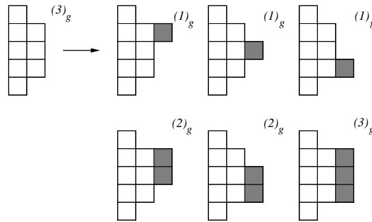
Fig. 7: The ECO operator for a polyomino in the class C_g .
