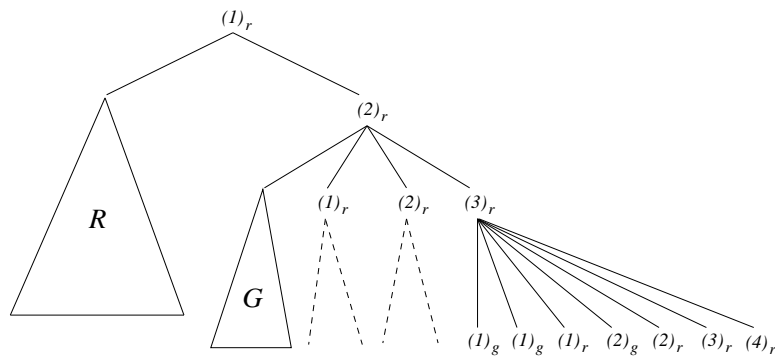
Fig. 9: The first levels of the generating tree of \Omega' .
