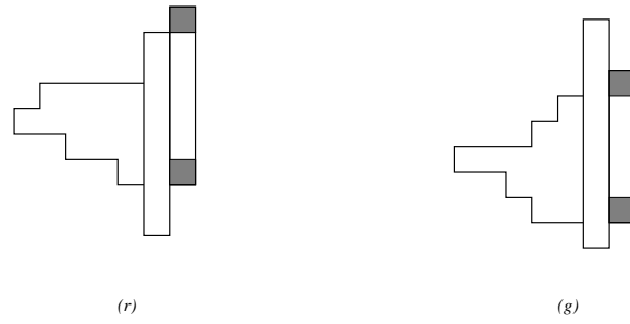
Fig. 3: Convex polyominoes in C_r , (r), and C_g , (g).
