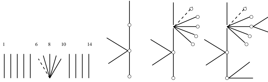
Fig. 5: Construction of trees of T_{14} with h = 6 and b - 2 = 6 .
