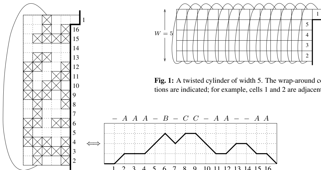
Fig. 2: Left: A snapshot during the construction of a polyomino. Everything to the left of the solid boundary line is already determined. This state has the connected components \{2, 3, 4, 11, 12, 15, 16\} , \{6\} , \{8, 9\} . Note that the bottom cell of the second column is adjacent to the top cell of the third column. The numbers are the labels of the boundary cells. Right: the same state encoded by assigning a distinct letter to each component and using the symbol “-” for empty cells, and the corresponding Motzkin path (0, 1, 0, 0, 1, 1, -1, 1, 0, -1, -1, 0, 1, 0, -1, 0, -1) .
