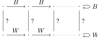
Figure 1: Illustration of the example fixpoint formula
