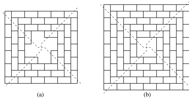
Fig. 4: Graphs of non-fixed edges for (a) \mathcal{A}_{QT}(12, bbbaaa) (b) \mathcal{A}_{QT}(14, bbbcaaa)
