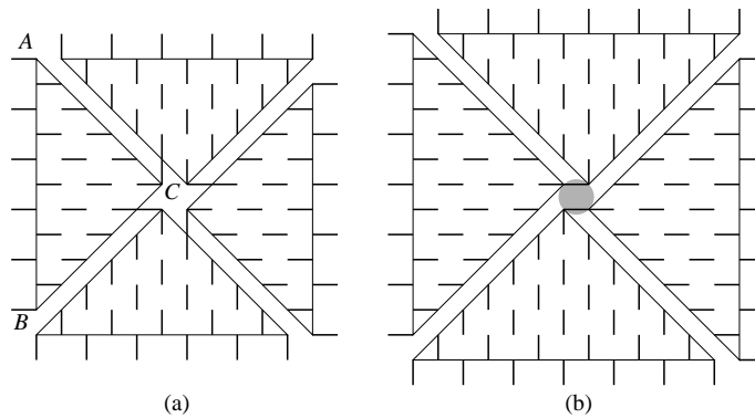
Fig. 3: Fixed edges for (a) \mathcal{A}_{QT}(12, bbbaaa) (b) \mathcal{A}_{QT}(14, bbbcaaaa)
