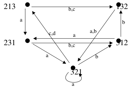
Fig. 3: The directed graph G(Av_4(123)) .
