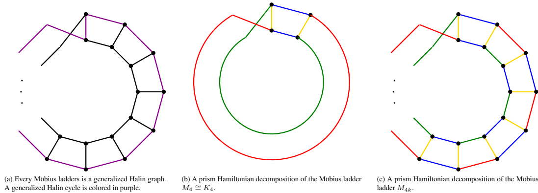
Fig. 12: Möbius ladders are prism-decomposable.
