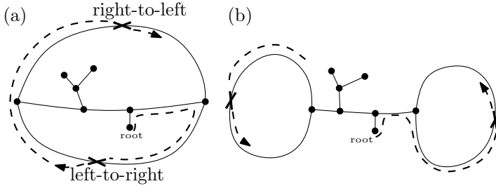
Fig. 5: Two maps on the Klein Bottle. (a) T_{LR}(m) = 1, T_{RL}(m) = 1 ; (b) T_{LR}(m) = 2, T_{RL}(m) = 0 .
