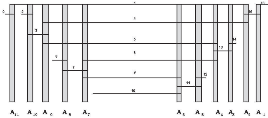
Fig. 1: The interval representation given by Tze-Heng Ma [39].
