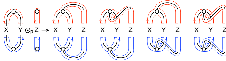
Fig. 13: ss'_i \odot_p uu'_j \rightarrow 4g_{i+j+1} .
