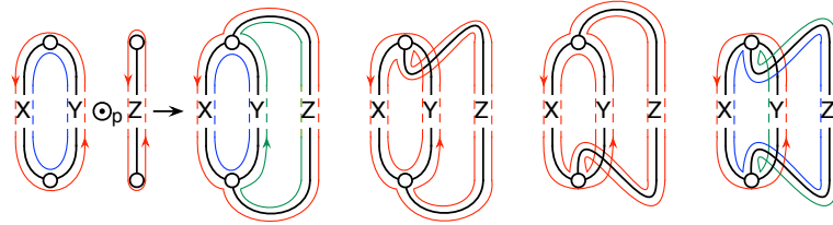
Fig. 12: dd''_i \odot_p uu'_j \rightarrow 2g_{i+j} + 2g_{i+j+1} .
