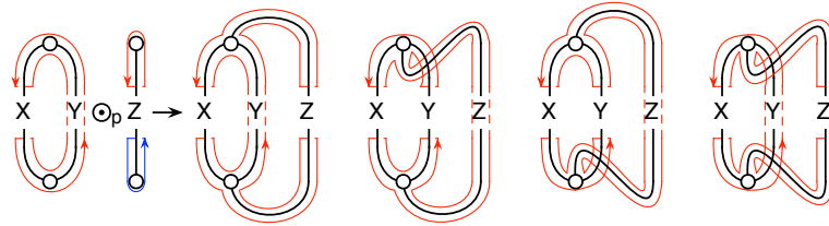
Fig. 15: ss'_i \odot_p uu_j \rightarrow 4g_{i+j+1} .
