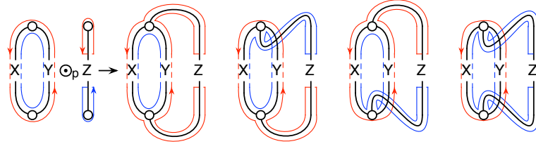
Fig. 11: dd''_i \odot_p uu'_j \rightarrow 4g_{i+j+1} .
