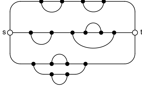
Fig. 9: A cubic series-parallel graph.
