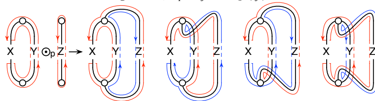
Fig. 16: ss'_i \odot_p uu'_j \rightarrow 4g_{i+j} .
