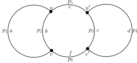
Fig. 1: A generalized polygon tree with three interior regions.
