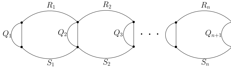
Fig. 3: A family of 2-connected bipartite graphs with no VC \{a, b\} -EW.
