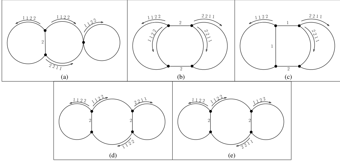
Fig. 2: A VC 2-EW for G .
