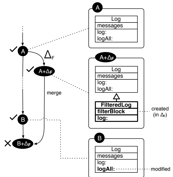
Figure 1. A developer starts a new branch of the library from version A of a logging library and implements a new feature: the FilteredLog . We name such change as \Delta_F . Before \Delta_F is integrated into the library, a modification in the method Log \gg logAll: in B makes B + \Delta_F not working.
