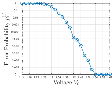
Figure 1: Set of voltages of an FPGA multiplier block and the associated error probabilities measured on random inputs at 90MHz and 27°C [4].
