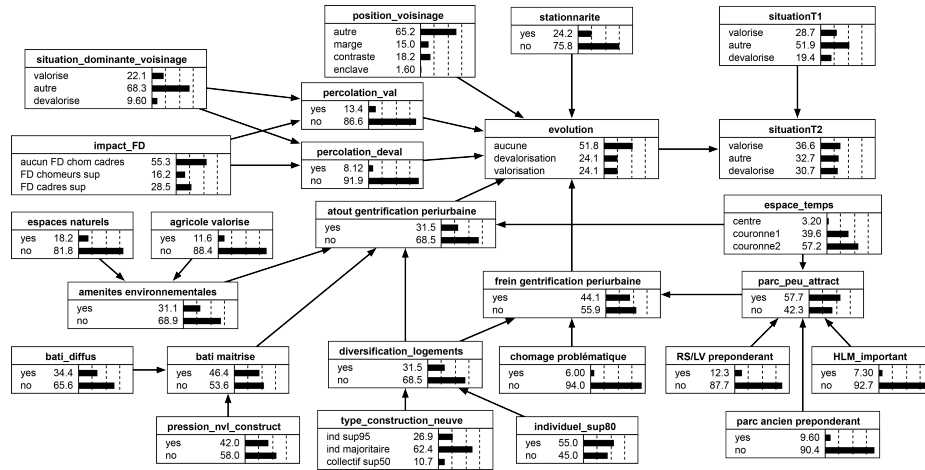
Fig. 1. The BN model for the valorization/devalorization of municipalities of the study area (from [15]).
