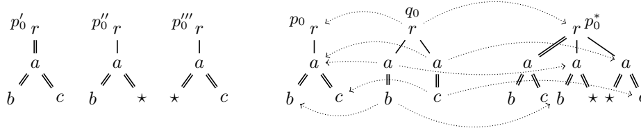
■ Figure 11 Immediate anchored generalizations versus an embedding with overlap p_0 \triangleleft_o q_0 .
