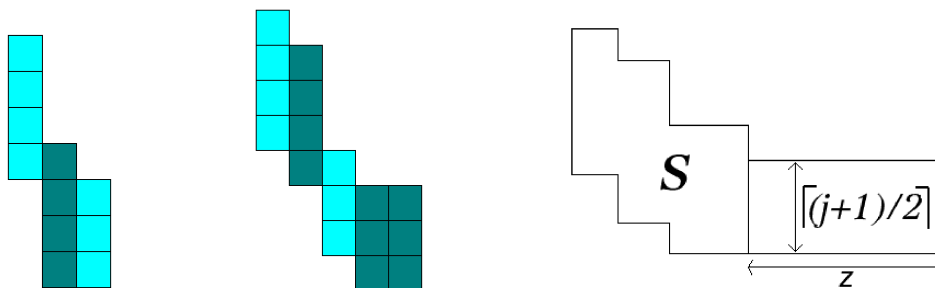
Fig. 4: Partial 6-shape s . Fig. 5: Partial 6-shape s \oplus_1^6 3^2 . Fig. 6: Gluing of the rectangle \lceil (j + 1)/2 \rceil^{z_j} to s .
