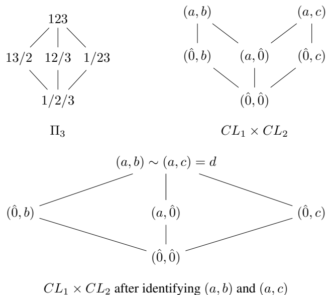
Fig. 2: Hasse diagrams for the partition lattice example
