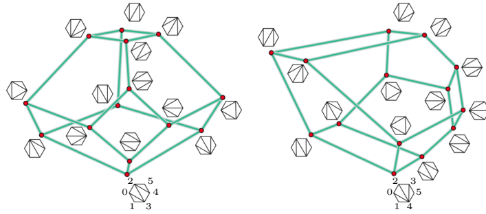
Fig. 1: Two 3-dimensional associahedra As_3^\xi = P_4(\{\tilde{z}_f^\xi\}) with vertex coordinates computed for differently chosen Coxeter elements according to [HL07] after application of an orthogonal transformation. The different Coxeter elements are encoded by different labelings of hexagons as indicated.
