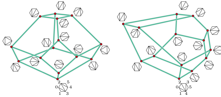
Fig. 1: Two 3-dimensional associahedra As_3^\xi = P_4(\{\tilde{z}_I^\xi\}) with vertex coordinates computed for differently chosen Coxeter elements according to [HL07] after application of an orthogonal transformation. The different Coxeter elements are encoded by different labelings of hexagons as indicated.
