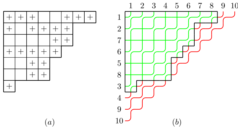
Fig. 1: A 2-north-east filling of \lambda = (8, 6, 6, 5, 4, 4, 1) and its associated reduced pipe dream.
