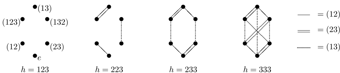
Fig. 3: Moment graphs of regular semisimple Hessenberg varieties.
