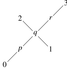
Figure 2: A marked Hasse diagram defining a partial order on the set P = \{p, q, r\} \cup A with |A| = 4 and \lambda = (3, 2, 1, 0) \in \mathbf{R}^A .
