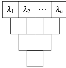
Figure 1: Board defining Gelfand–Tsetlin patterns.
