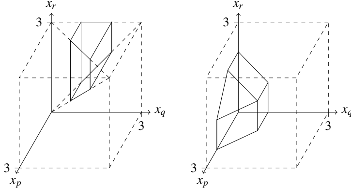
Figure 3: The marked order polytope of the marked poset in Figure 2 is given by the inequalities 0 \leq x_p \leq x_q \leq x_r \leq 3 and 1 \leq x_q \leq 2 . The marked chain polytope is given by the inequalities x_p, x_q, x_r \geq 0 , x_p + x_q + x_r \leq 3 , x_p + x_q \leq 2 , x_q + x_r \leq 2 , and x_q \leq 1 . Note that they are not combinatorially isomorphic.
