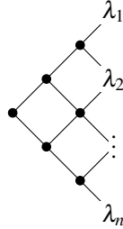
Figure 4: Marked Hasse diagram for \mathfrak{sl}_n .
