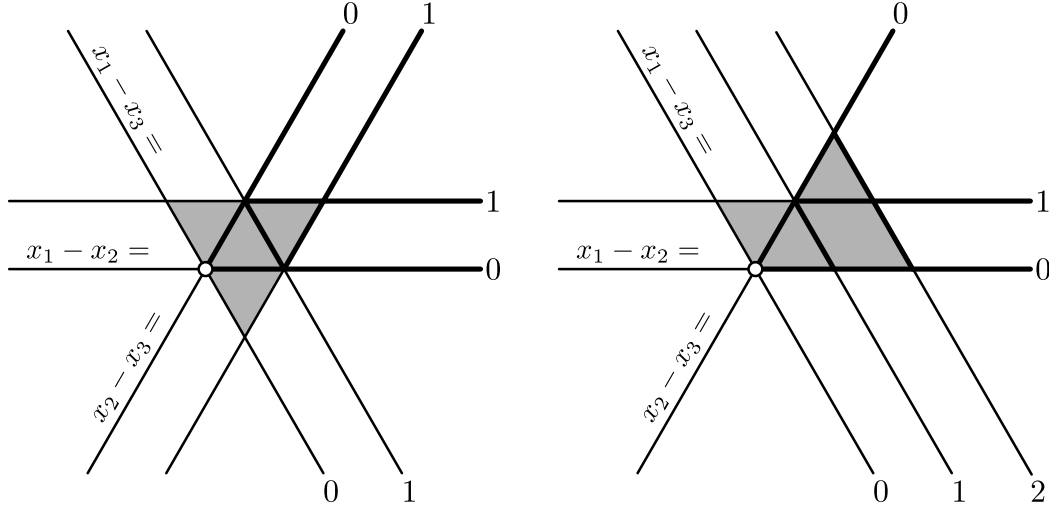
Fig. 1: The arrangements \text{Shi}(3) (left) and \text{Ish}(3) (right)
