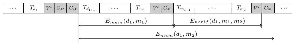
Figure 2: Placing memory checkpoints.
