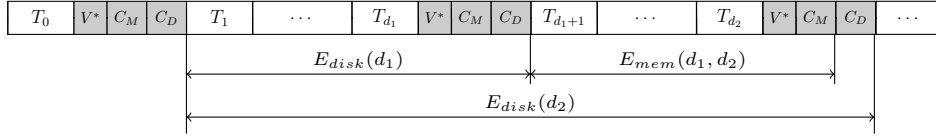
Figure 1: Placing disk checkpoints.
