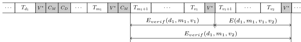
Figure 3: Placing verifications.
