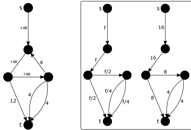
(a) capacities (b) loop-free flow
