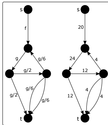
(a) capacities (b) loop-free flow
