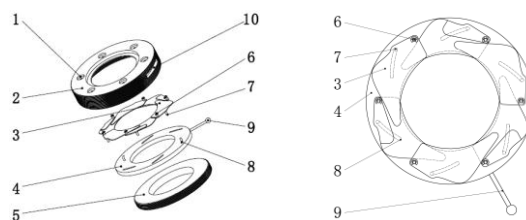
1. hole of hinge axis 2. blade connection seat 3. blade 4. cam ring 5. locked ring 6. hinge axis 7. sliding limited post 8. guiding chute 9. Handle 10. Notch of the connection seat
