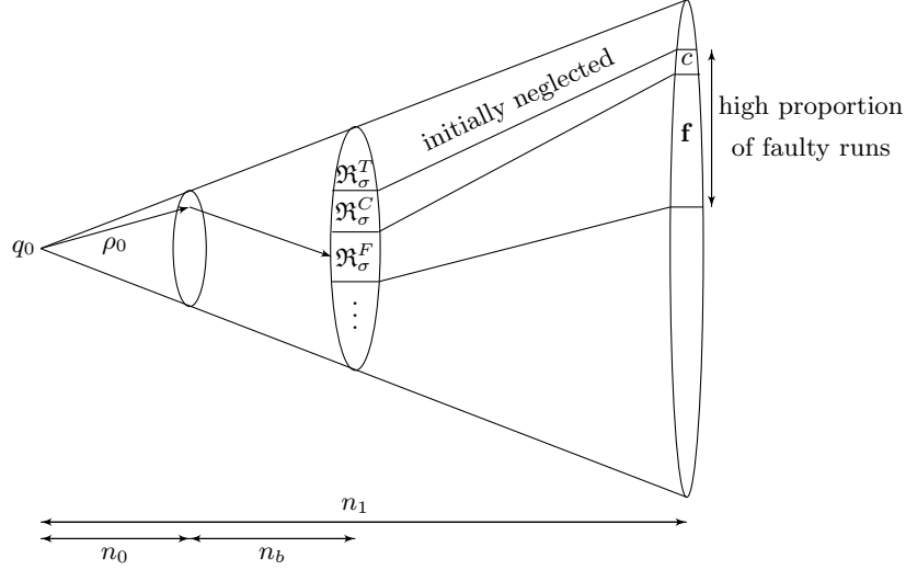
Fig. 5. Illustration of the proof of Lemma D.
