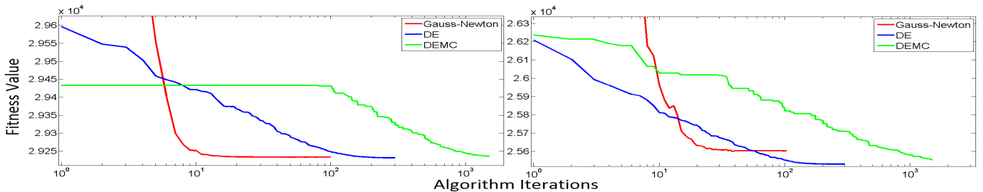
Fig. 3. Median fitness evolution for each optimization method in rats 1 (left) and 10 (right), respectively. We have zoomed-in on a sub-interval to get the nuances of the error evolution.
