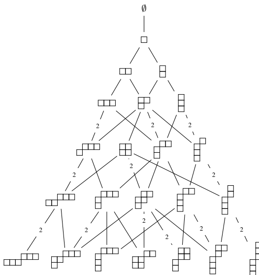
Fig. 2: The 4-core lattice up to rank 6. Only boxes with hook-lengths \neq 4 are drawn.
