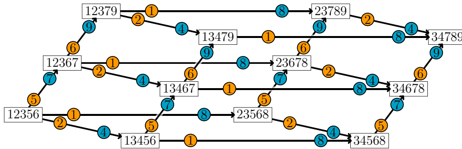
Fig. 2: The positive and negative edge labelings p and n of \mathcal{G}(Q^{\text{ex}}, \rho^{\text{ex}}) . Each edge has its positive label on the left (orange) and its negative label on the right (blue).
