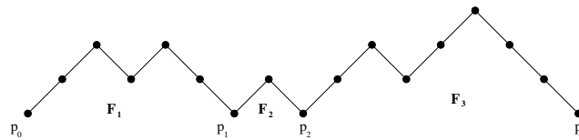
Fig. 1: A Dyck path having three factors.
