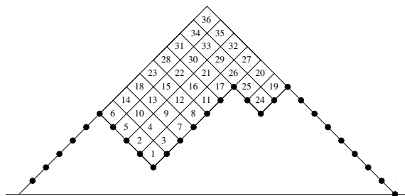
Fig. 7: The standard Young tableau determined by a Dyck path.
